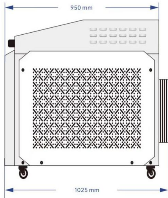
Side size
