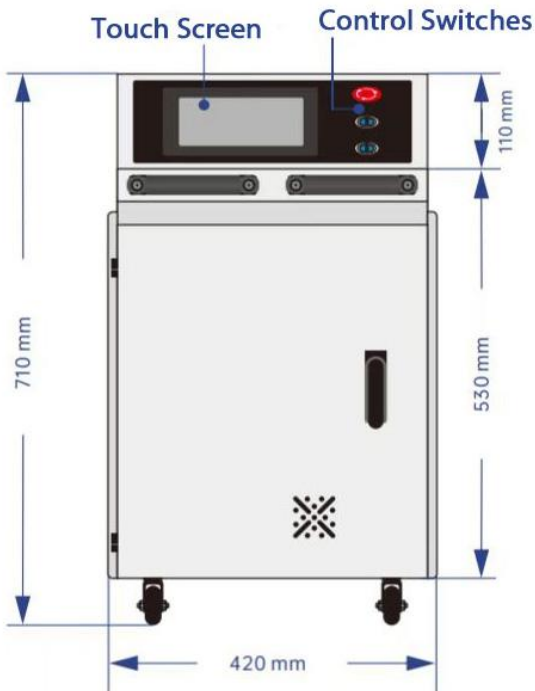
Front Size
